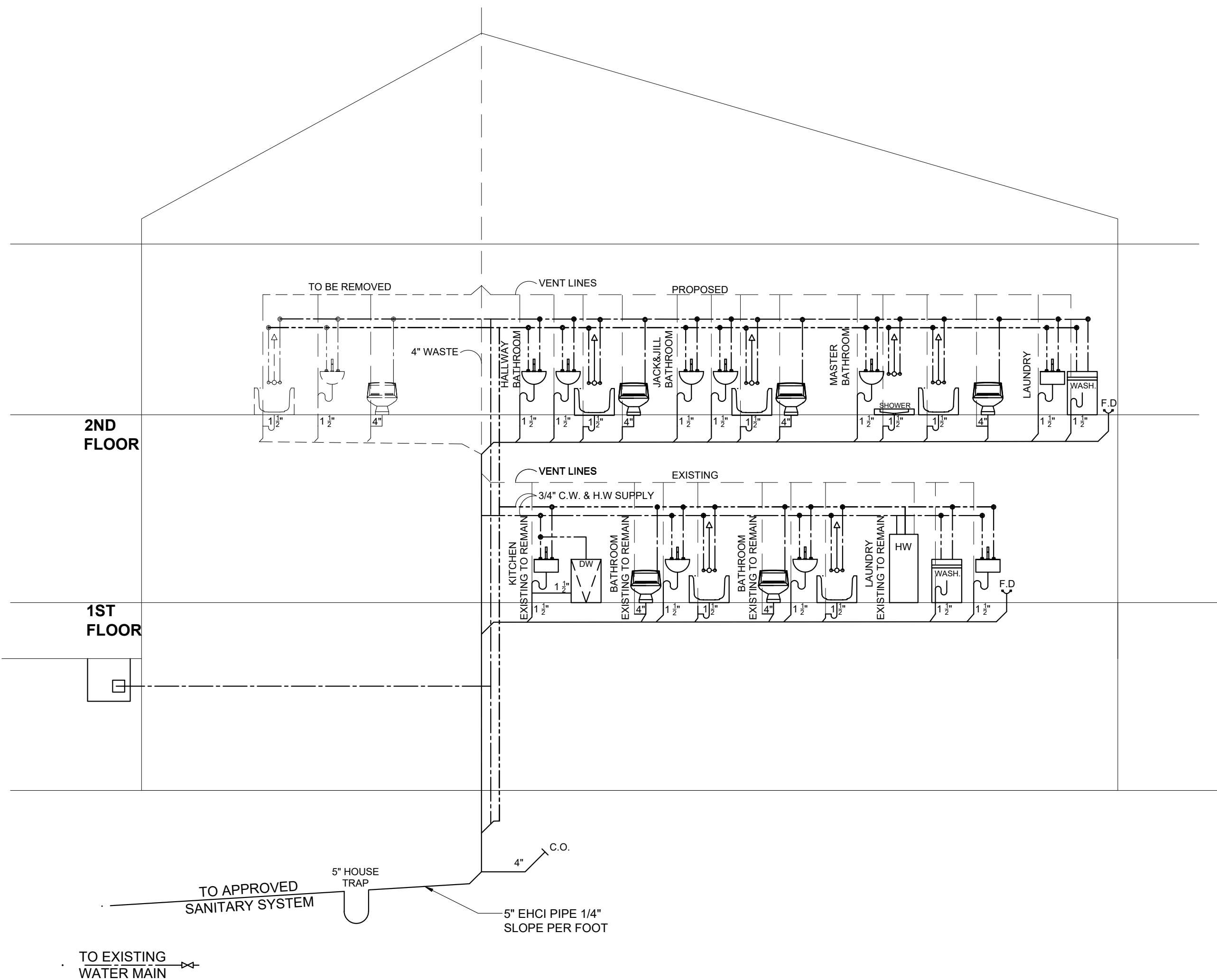
PLUMBING RISER DIAGRAM
