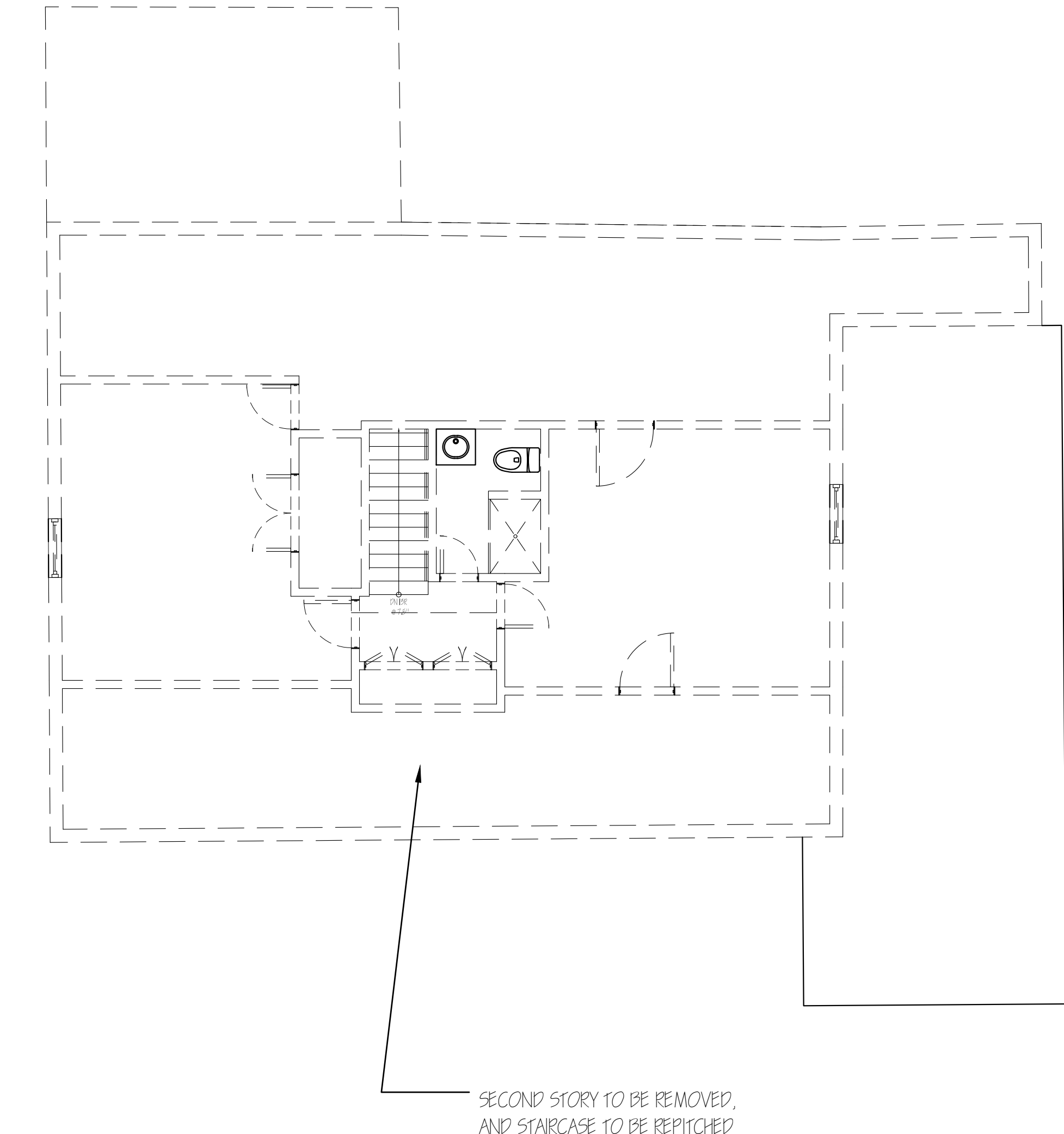
SECOND FLOOR PLAN (DEMOLITION) SCALE 3/16"=1'-0"
